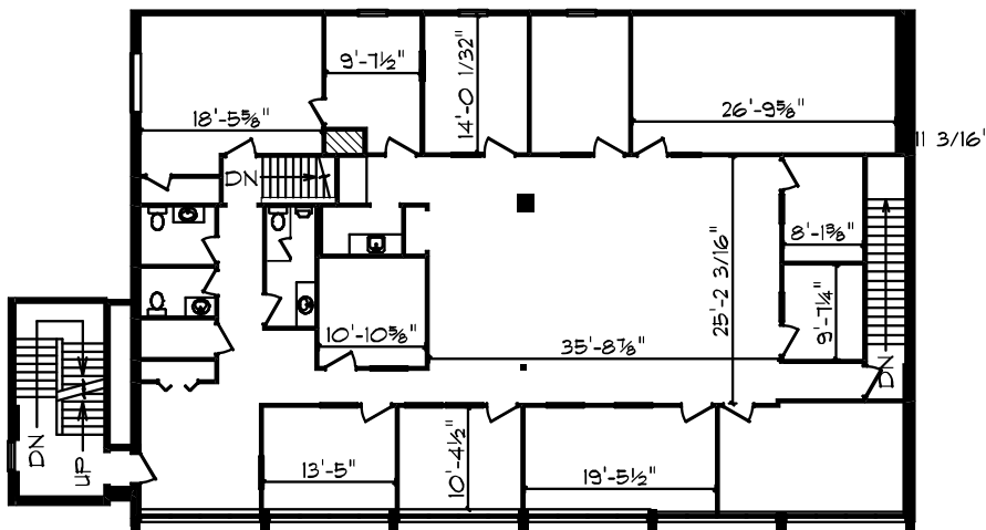
2ND FLOOR
